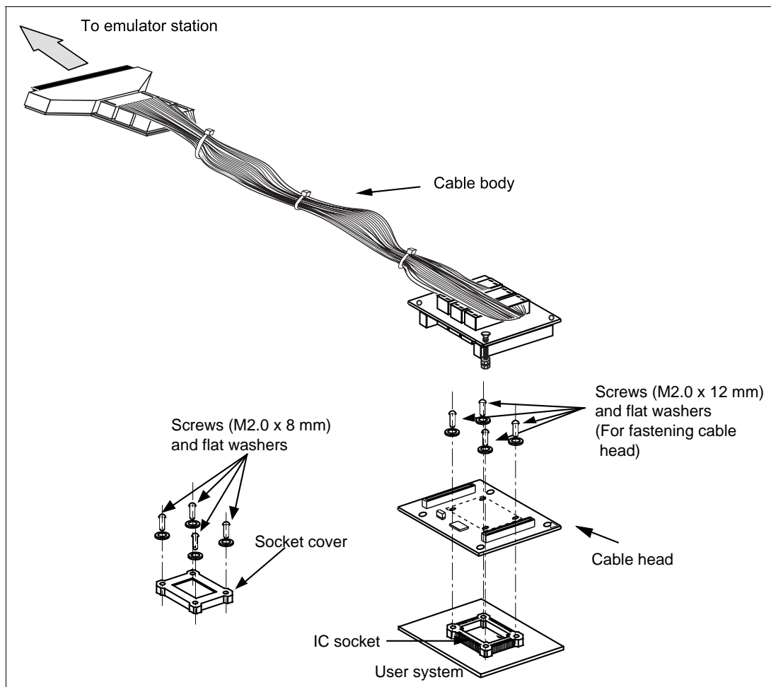
Figure 1 HS3257ECH61H User System Interface Cable
